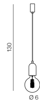
Volta 1 AZ2384 E27 1x MAX 40W concrete
